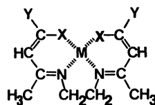
4 X=O, Y=Ph 5 X=S, Y=Ph 6 X=S, Y=CH 3
